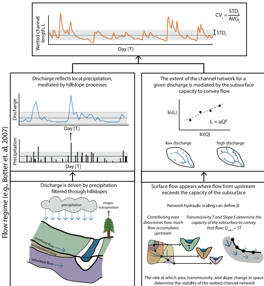
FIGURE 1 Flow regime (left) and network hydraulic scaling (right) co-determine the extent of and variation in wetted channel length through time (top). Hillslope runoff generation processes “filter” precipitation events leading to time variation in discharge (left), which is delivered to the channel network. The area-dependent scaling of discharge determines the magnitude of flow delivered to the channel at any point in the stream network, and transmissivity and slope determine the capacity of the channel subsurface to convey that flow (bottom right). Where discharge exceeds this subsurface capacity, surface flow emerges, resulting in a wetted channel. The relationship between flow and wetted channel length at the catchment mouth is observed to exhibit power law scaling: L = \alpha Q^\beta (center right). The timeseries of Q and the power law relationship between Q and L result in a timeseries of L (top) and its associated relative variability, CV_L
